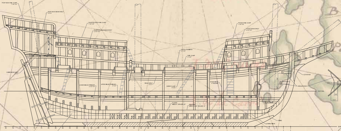
ELEVATION B-5 CONSTRUCTION PROFILE
