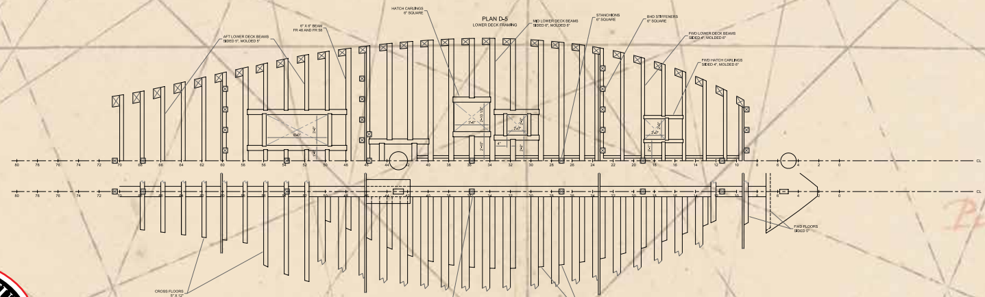
PLAN B-5 BOTTOM FRAMING
